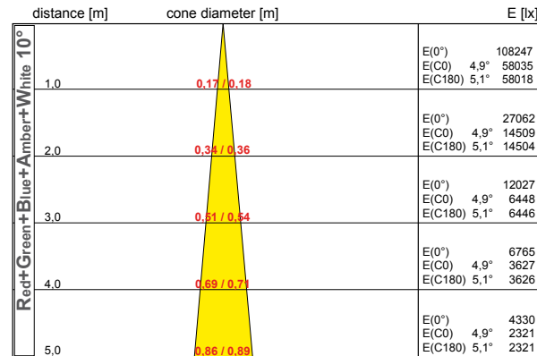
half value angle C0-180 : 9,8° C90-270 : 10,2° 132xLED, total flux: 7488,0 lm, LOR: 73%
